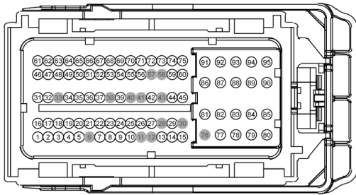
Rear Harness
